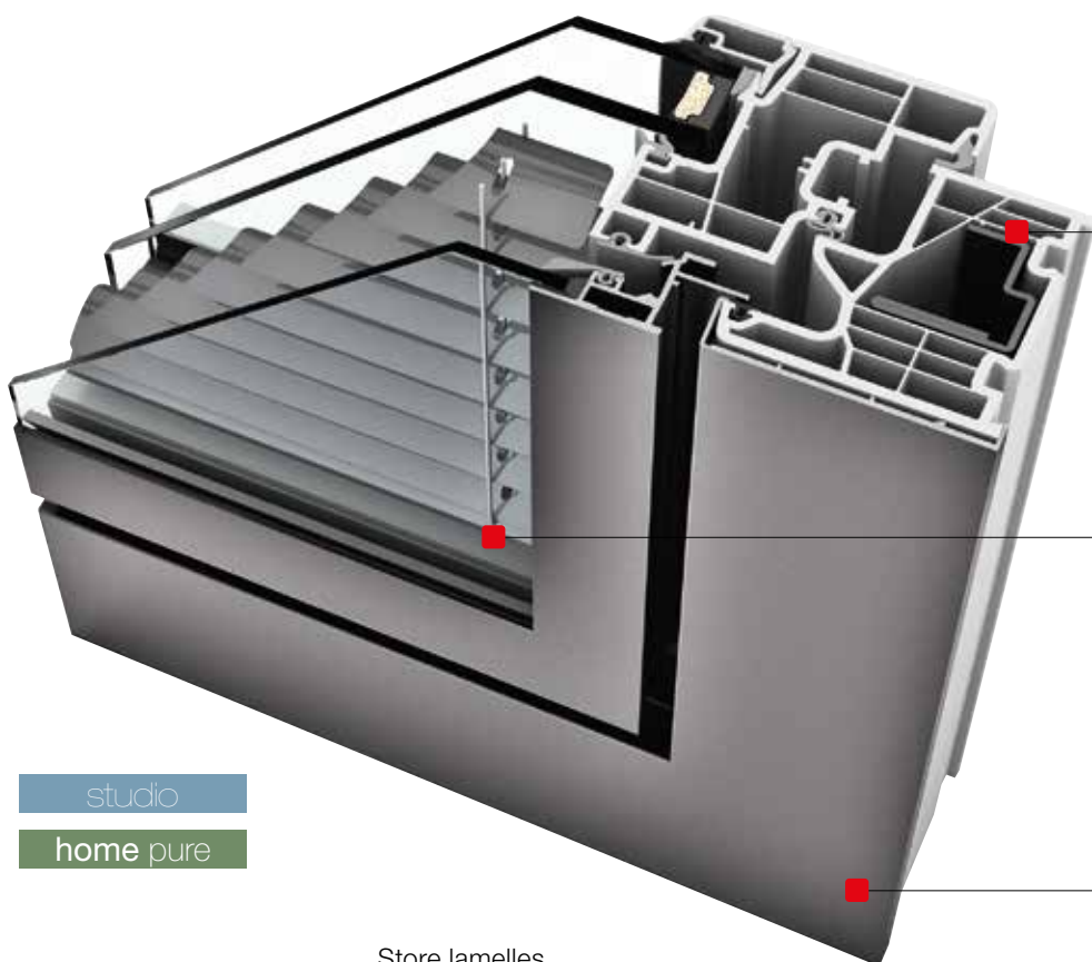
Store lamelles
